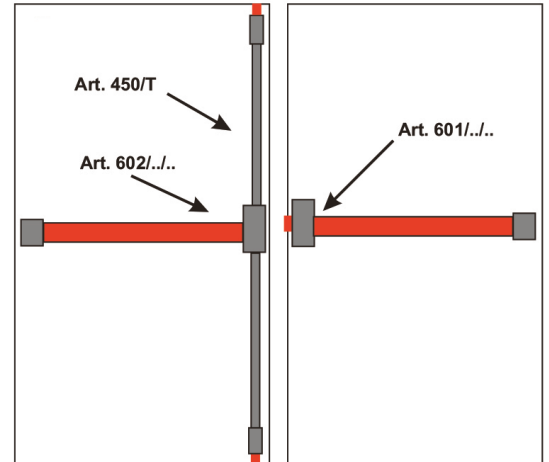
2066 Push bar double panic exit device
