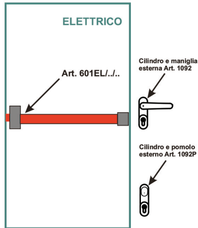
2065 Push bar single panic exit device
